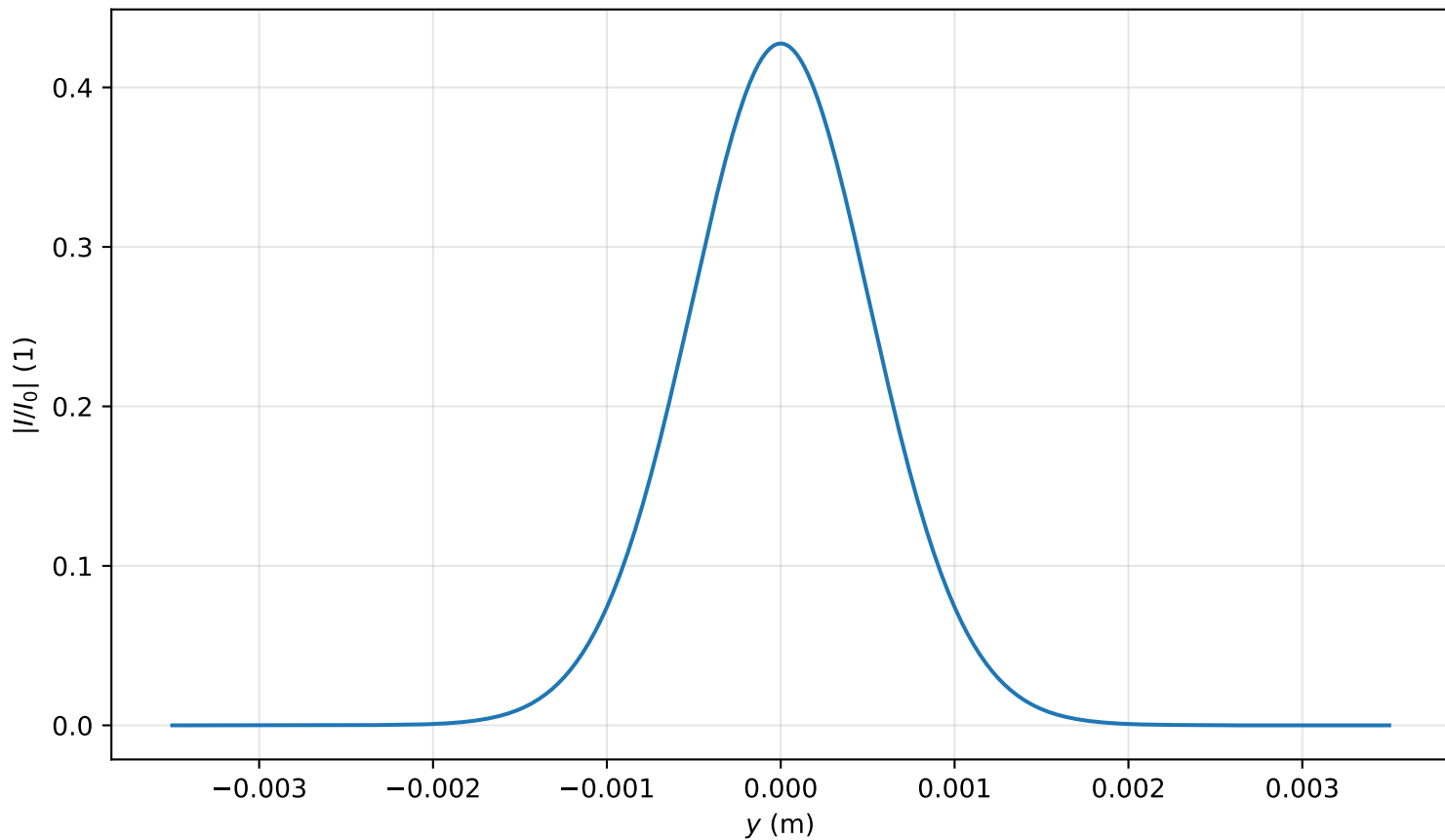
Intensity profile I(x=0, y, z=2.707)/I_0 , P_{in}=0.2P_{cr} , artificial time
